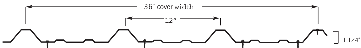
Cross section of Everlast PBR Panel
