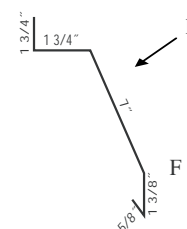
Ⓞ 29 Ga. Track Cover Cannonball FM 10'2" TLCT15xx
