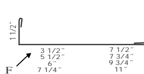
Ⓛ 29 Ga. Post Trim 10'2" TLPT10xxxx
