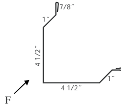
Ⓑ 29 Ga. Rake & Corner 10' 12' 14' 16' TLRC2xxxx
