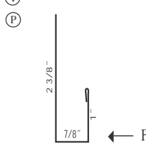
Ⓖ 29 Ga. "J" Channel 10'2" TLJC6xx
